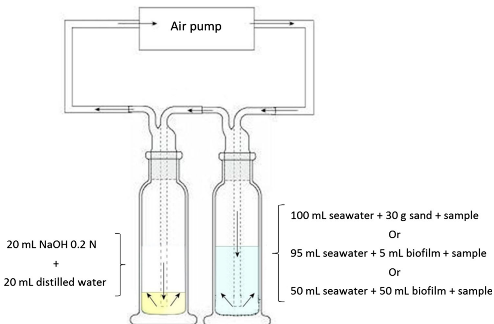
Fig. 2 Schema of biodegradation test at solid/liquid state and at liquid state in marine environment
