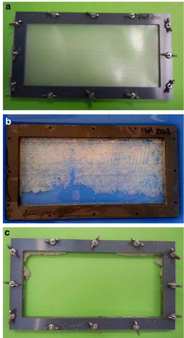
Fig. 4 PHBV specimen before (a) and after 6 and 9 months of immersion in natural seawater (b and c, respectively)
