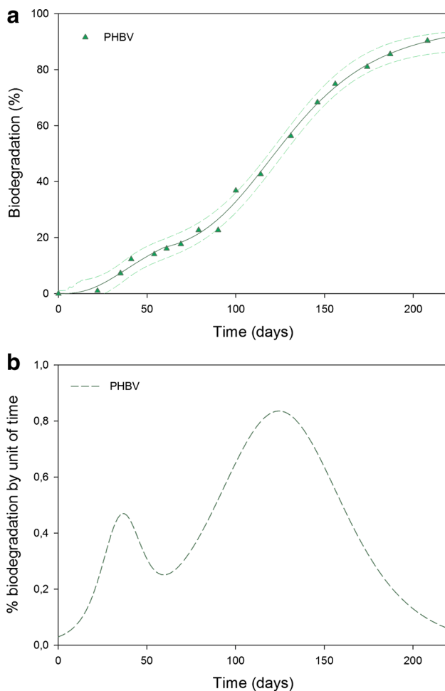
Fig. 7 Biodegradation test of PHBV and cellulose powders in inoculated foreshore sand (the solid line shows the degradation curve, which was calculated with the Hill and Boltzmann model and the short lines correspond to the probability that 95 % of the values are within these intervals) (a) and evolution of the microbial activity (b)
