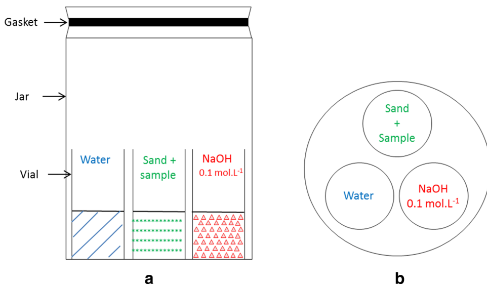
Fig. 1 Schema of biodegradation test at solid state in foreshore sand: a front view and b top view
