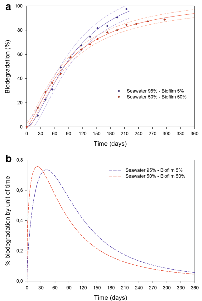
Fig. 8 Biodegradation test of PHBV and cellulose powders in inoculated seawater and foreshore sand (the solid line shows the degradation curve, which was calculated with the Boltzmann model and the short lines correspond to the probability that 95 % of the values are within these intervals) (a) and evolution of the microbial activity (b)
