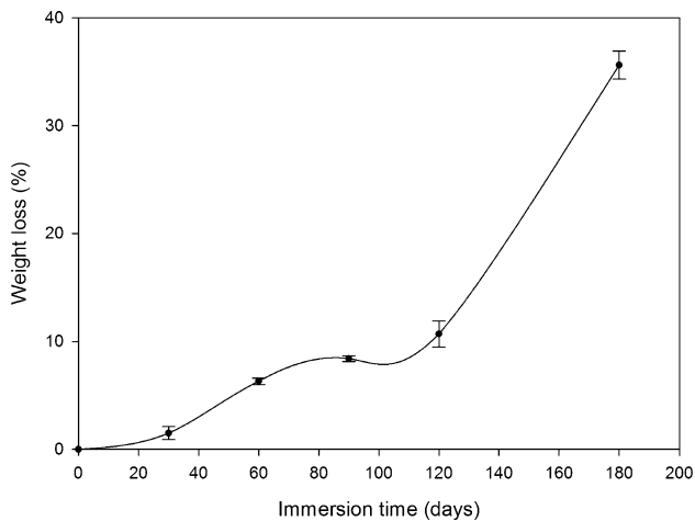
Fig. 3 Evolution of weight loss as a function of immersion time for the PHBV film aged in natural condition (and error bars correspond to standard deviations)
