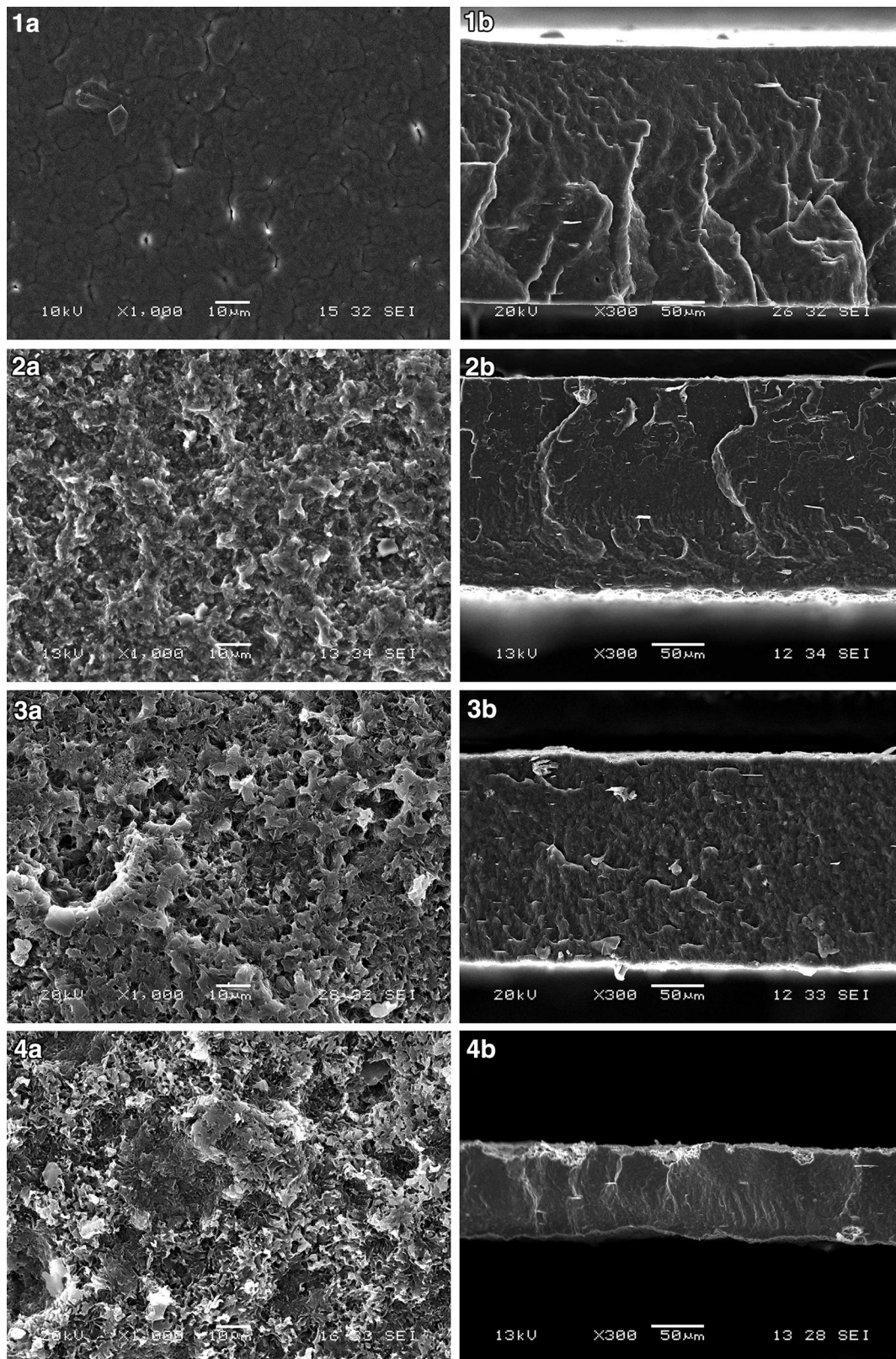
Fig. 5 SEM micrographs of the surface (a) and the fracture (b) of PHBV films unaged (1) and aged in natural seawater after 60 days (2), 120 days (3) and 180 days (4)
